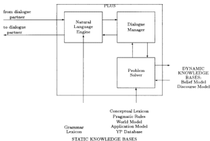
Figure 1: Outline Architecture
