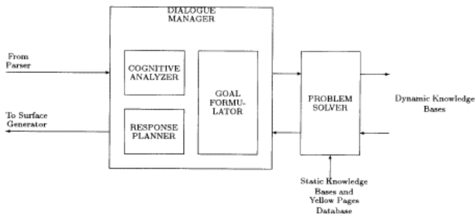
Figure 3: Dialogue Manager.
